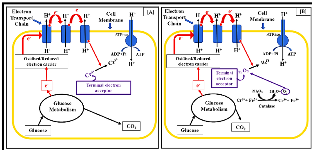
Figure 5.2.1: The schematic representation of predicted anaerobic respiration techniques implied by chromium resistant sewage dwelling microbes. [A] In Microbacterium radiodurans K12016, the hexavalent chromium directly behaving as terminal electron acceptor of respiratory electron transport chain (ETC). [B] In
